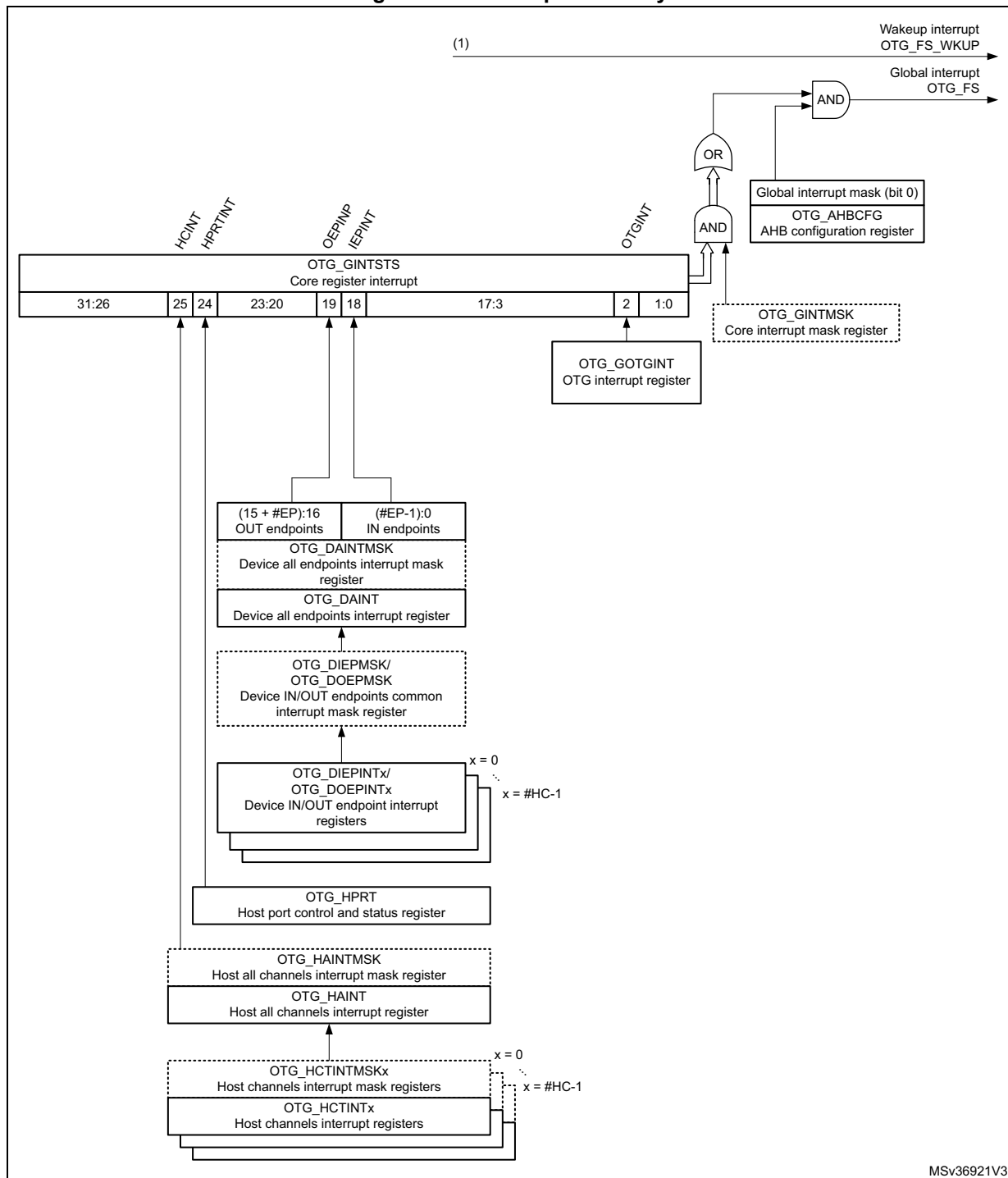
Figure 250. Interrupt hierarchy
